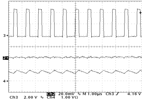
( V_{IN} = 5\text{ V} , I_{LOAD} = 700\text{ mA} , L = 3.3\ \mu\text{H} , C_{OUT} = 20\ \mu\text{F} ) Upper Trace: L_X Pin Switching Waveform, 2 V / div. Middle Trace: Output Ripple Voltage, 20 mV / div. Lower Trace: Inductor Current, 1 A / div.
