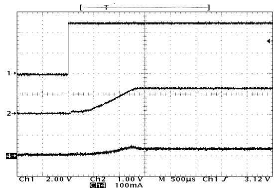
( V_{IN} = 5\text{ V} , I_{LOAD} = 100\text{ mA} , L = 3.3\ \mu\text{H} , C_{OUT} = 20\ \mu\text{F} \times 2 ) Upper Trace: Enable Pin Voltage, 2 V / div. Middle Trace: Output Voltage, 1 V / div. Lower Trace: Input Current, 100 mA / div.
