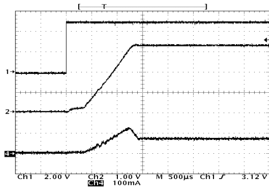
( V_{IN} = 5\text{ V} , I_{LOAD} = 100\text{ mA} , L = 3.3\ \mu\text{H} , C_{OUT} = 20\ \mu\text{F} \times 2 ) Upper Trace: Enable Pin Voltage, 2 V / div. Middle Trace: Output Voltage, 1 V / div. Lower Trace: Input Current, 100 mA / div.
