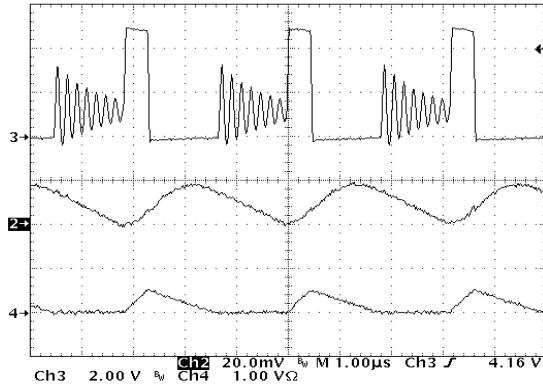
( V_{IN} = 5\text{ V} , I_{LOAD} = 100\text{ mA} , L = 3.3\ \mu\text{H} , C_{OUT} = 20\ \mu\text{F} ) Upper Trace: L_X Pin Switching Waveform, 2 V / div. Middle Trace: Output Ripple Voltage, 20 mV / div. Lower Trace: Inductor Current, 1 A / div.
